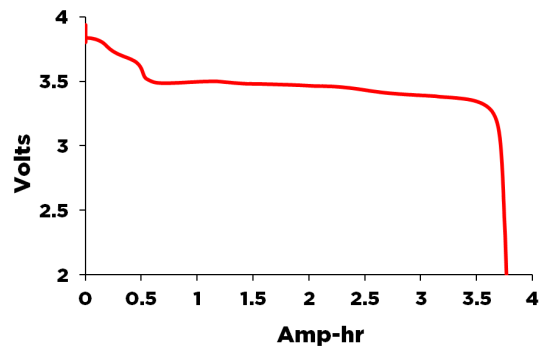
Discharge Curve 75 mA, 23°C
