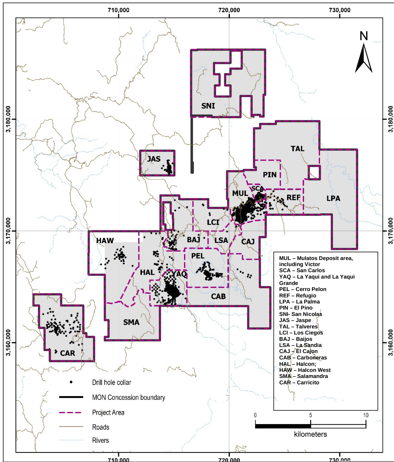
Figure 10-2 Post-2001 Drill Hole Locations
