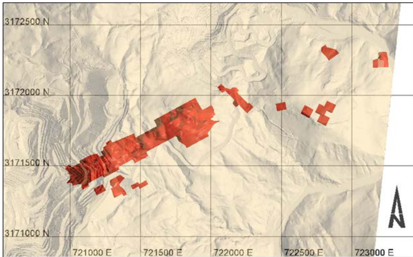
Figure 14-38 PDA - Wireframes – Plan View
