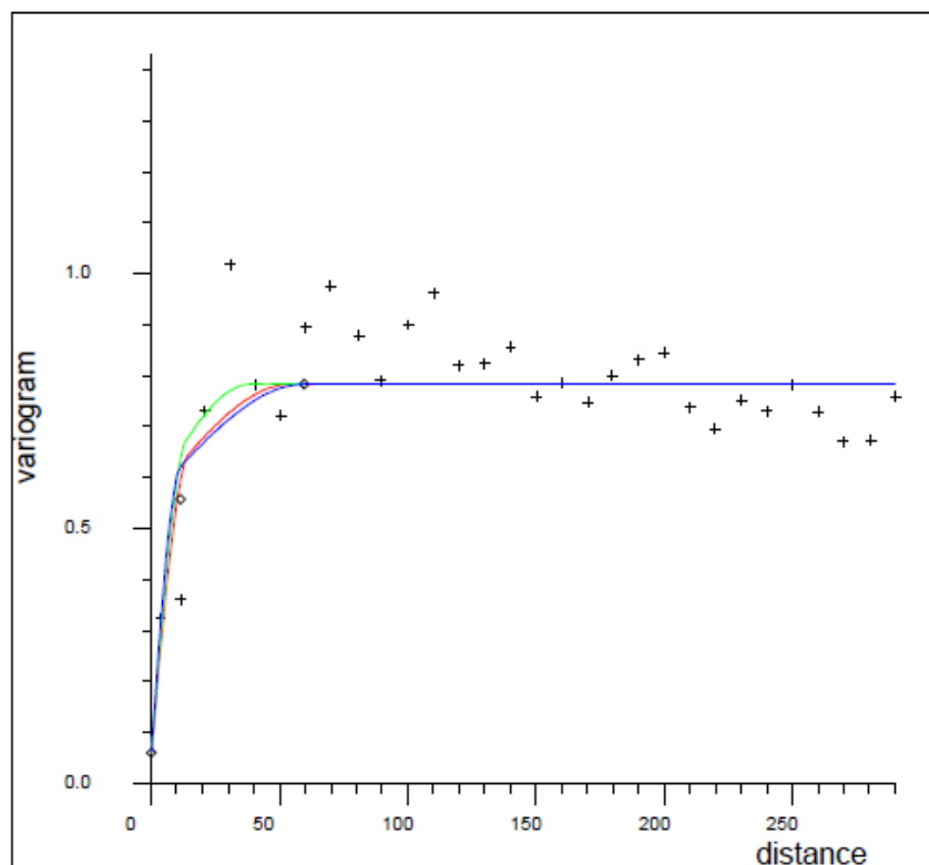
Figure A-6. Silver Variograms – Higher-Grade Silver Zone 2 – La Yaqui Grande
