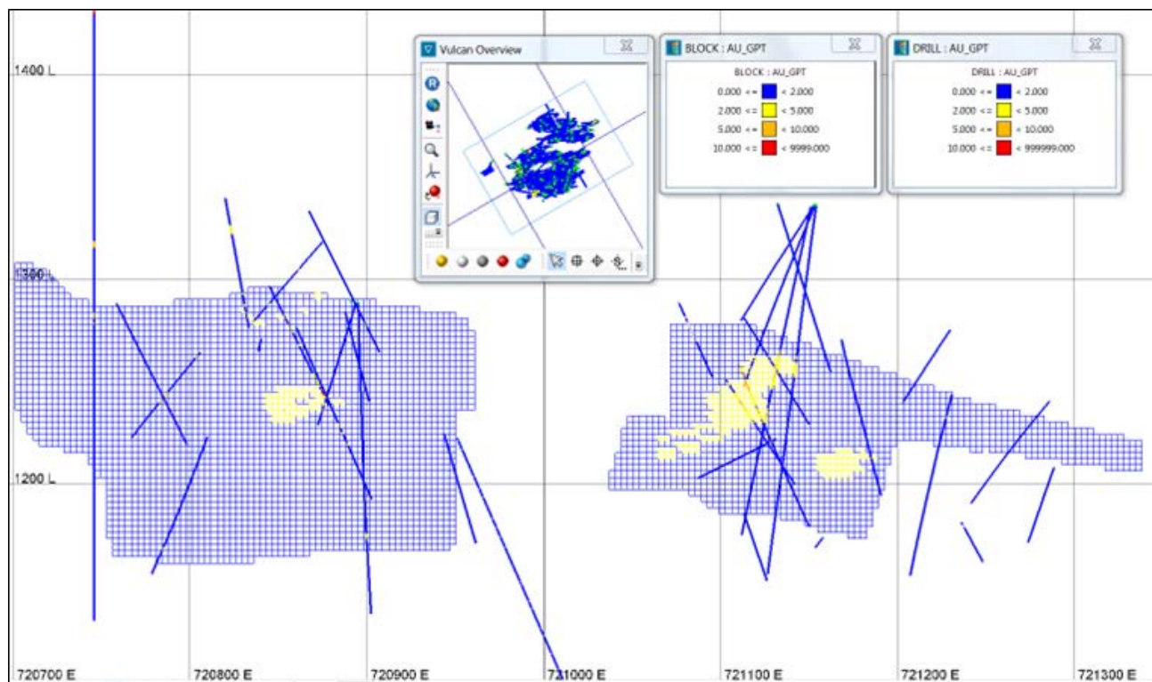
Figure 14-52 Estrella - Gold Grade Estimates and Drill Hole Gold Grades – Longitudinal NE-SW Section Looking NW
