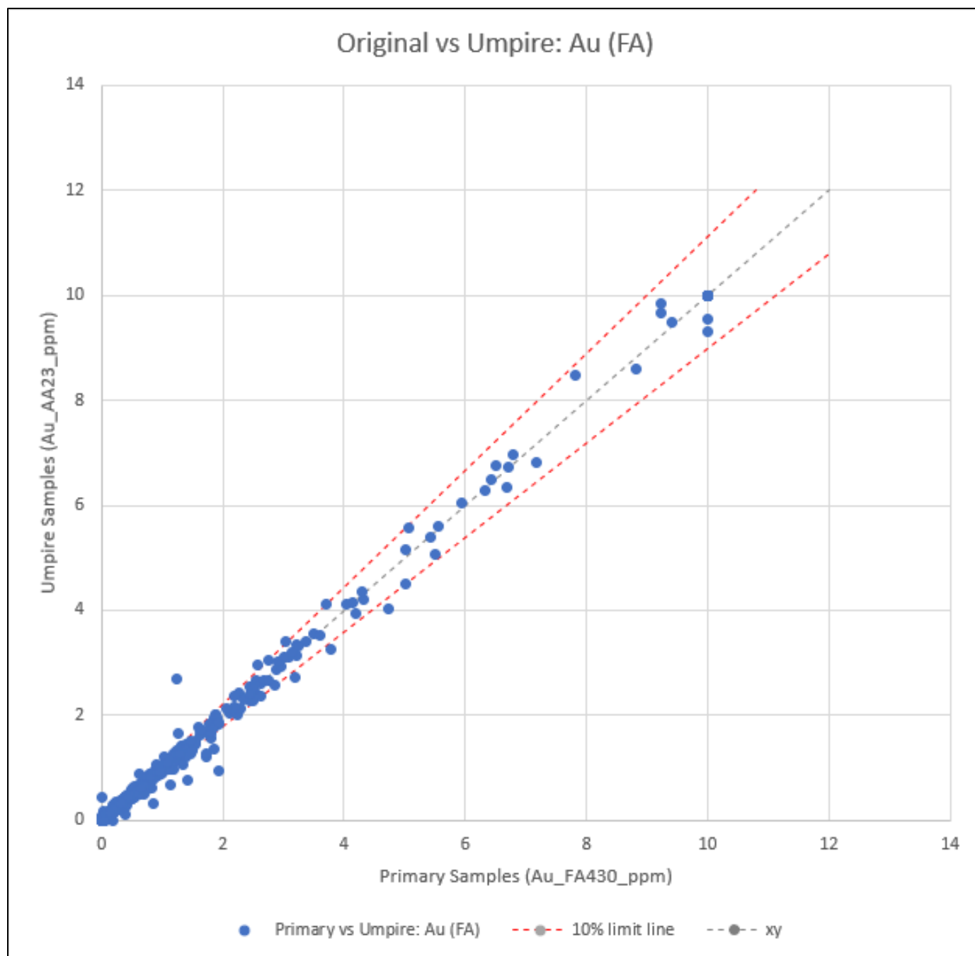
Figure 11-3 Scatter Plot of Check versus Original Assays from 2014-2022
