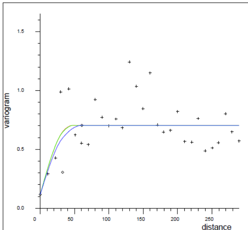
Figure A-5. Silver Variograms – Higher-Grade Silver Zone 1 – La Yaqui Grande
