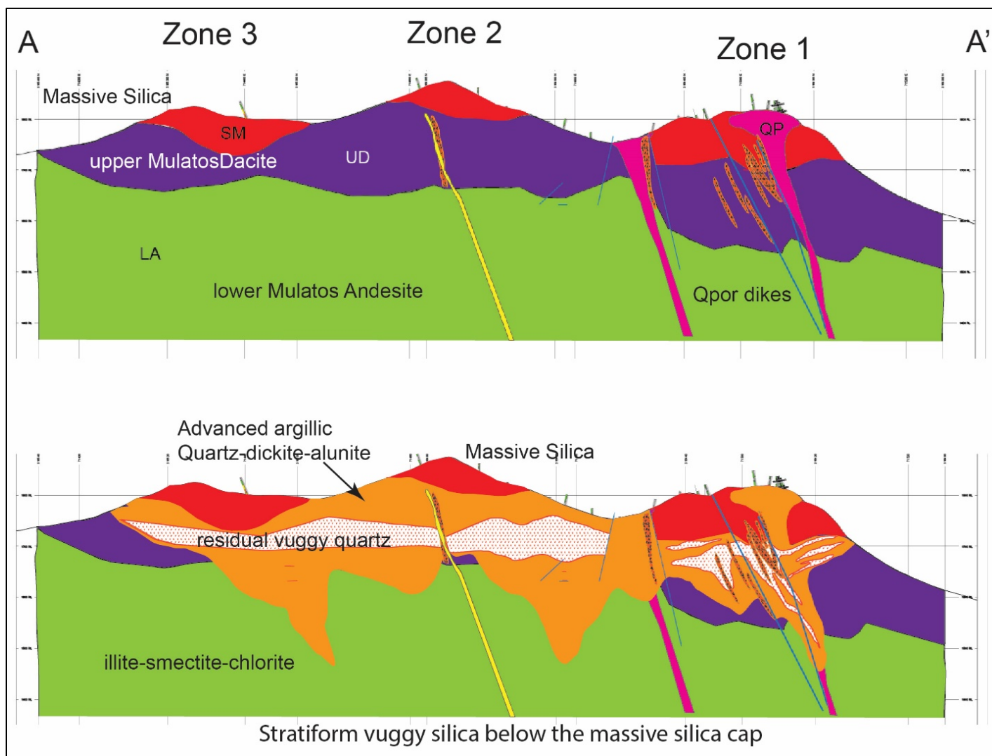
Figure 7-7 Geologic Cross Sections A-A' Showing Lithologies Above and Alteration Below.
