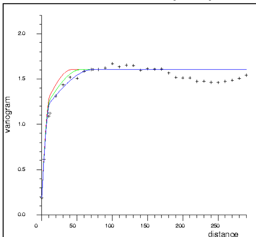
Figure B-1. Gold Variograms – PDA Sulphide Zone
