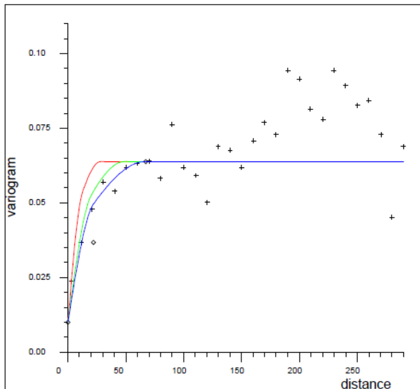
Figure A-9. AuCN/Au Variograms – Oxide – La Yaqui Grande
