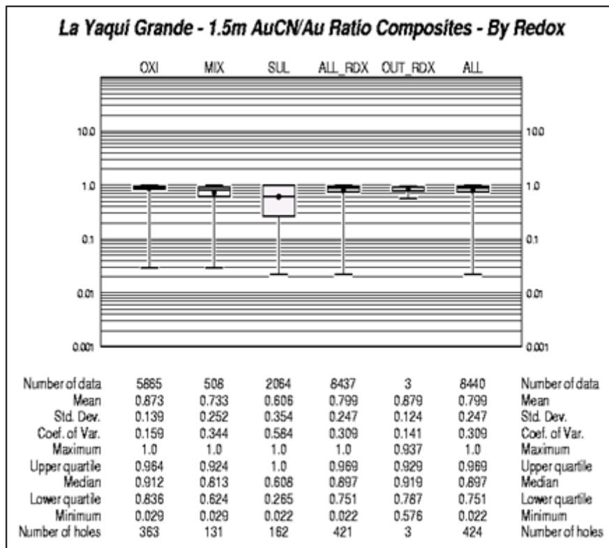
Figure 14-11 LYG - Boxplots of AuCN/Au Ratio Composites
