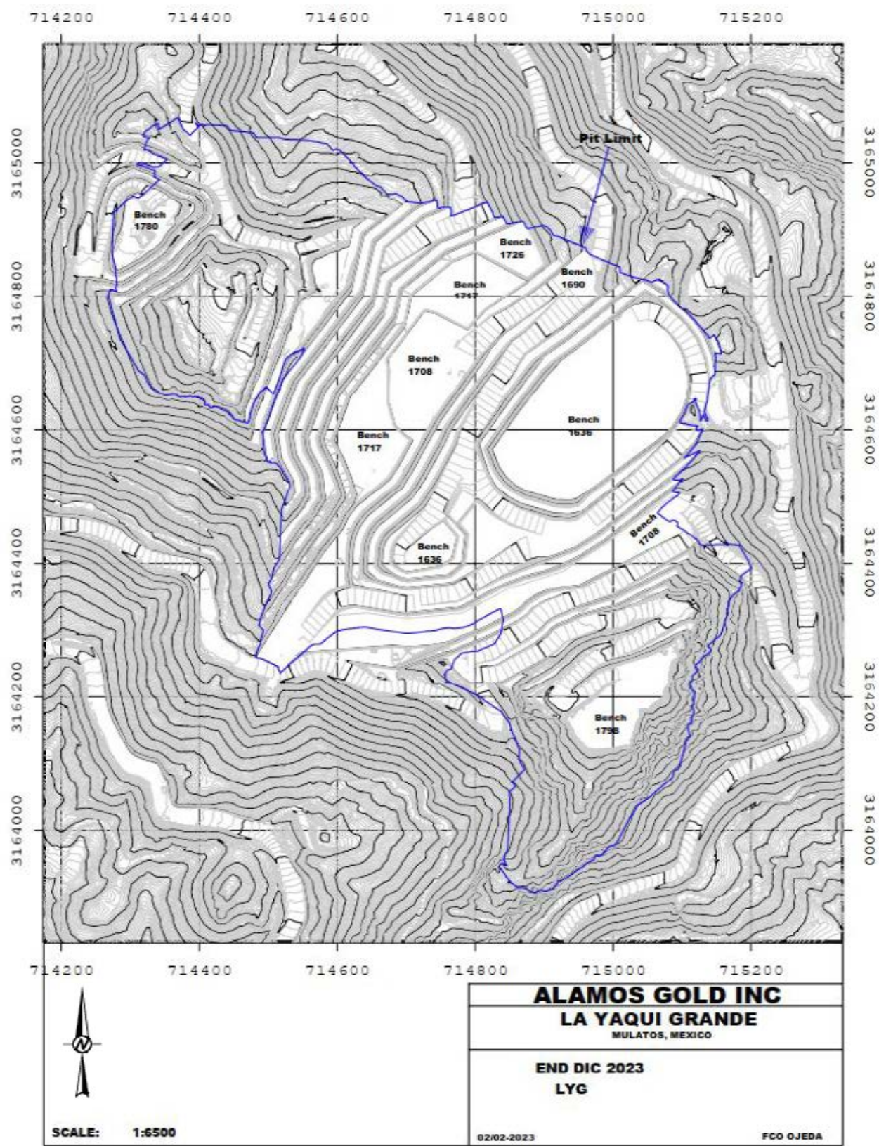
Figure 16-6 La Yaqui Grande Pit Plan, End of 2023
