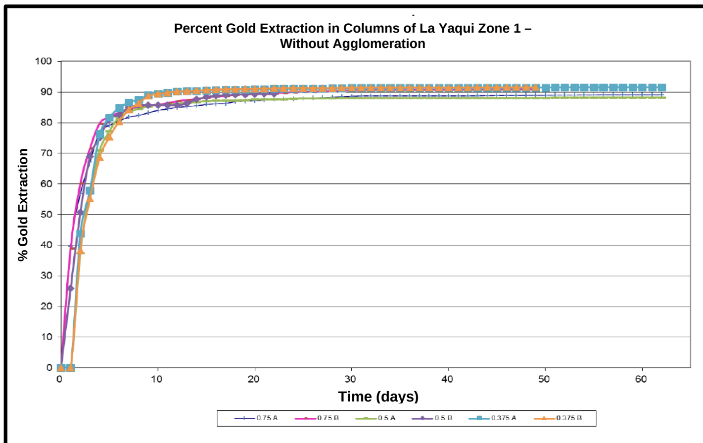
Figure 13-4 La Yaqui Grande Zone 1 Columns without Agglomeration
