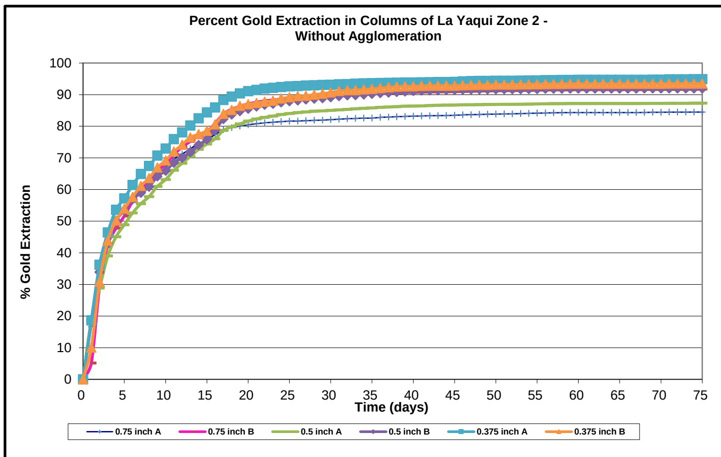
Figure 13-6 La Yaqui Grande Zone 2 Columns without Agglomeration
