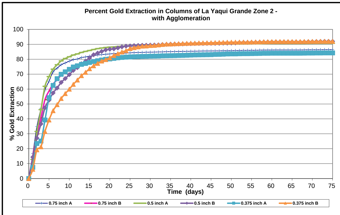
Figure 13-7 La Yaqui Grande Zone 2 Columns with Agglomeration
