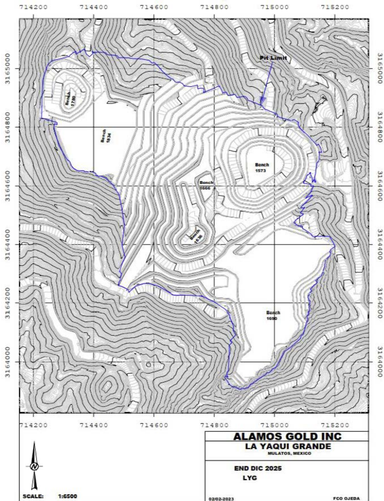
Figure 16-8 La Yaqui Grande Pit Plan, End of 2025
