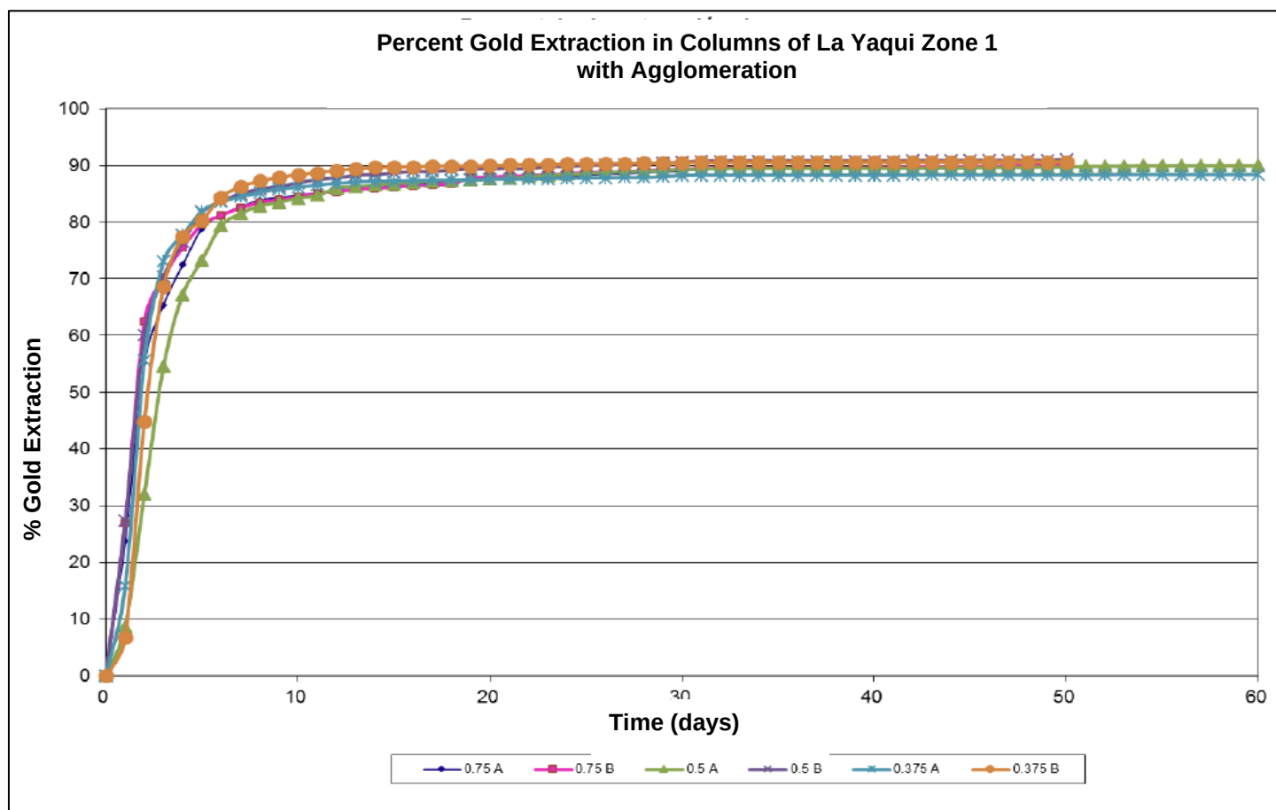
Figure 13-5 La Yaqui Grande Zone 1 Columns with Agglomeration
