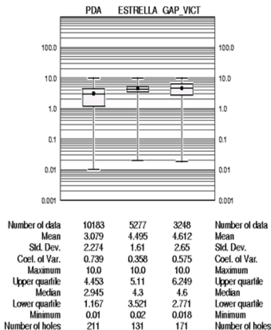
Figure 14-50 PDA Project - Boxplots of Total Sulphur Grade Composites – Capped – Within Mineralized Zones
