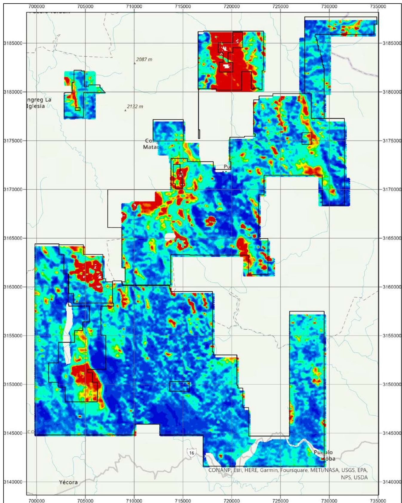
Figure 9-2 2018 VTEM Survey Showing Resistivity at a 50m Depth Slice
