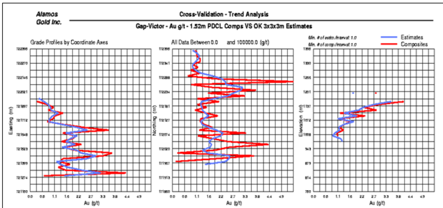
Figure 14-56 Gap-Victor - Gold Grade Profile
