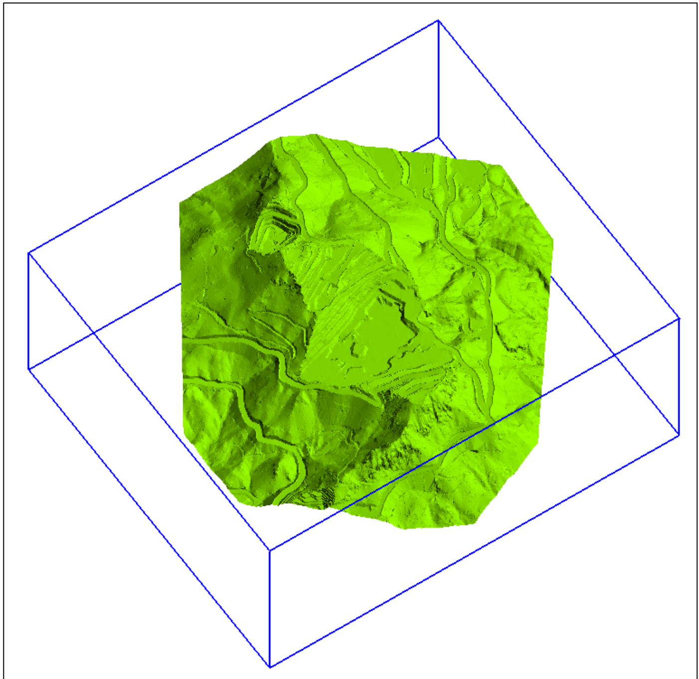
Figure 14-27 LYG – Mined-Out Topography Surface as of December 31, 2022 – Looking North
