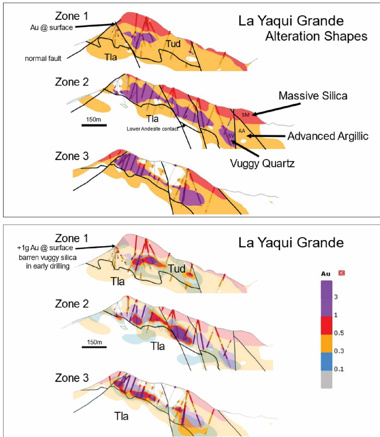
Figure 7-9 Modelled Cross Sections through Zones 1-3 of the La Yaqui Grande Deposit
