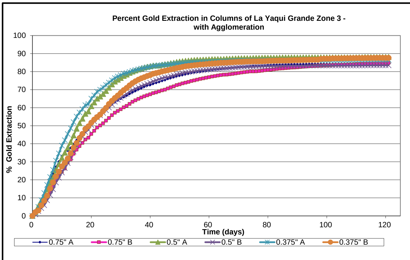
Figure 13-9 La Yaqui Grande Zone3 Columns with Agglomeration
