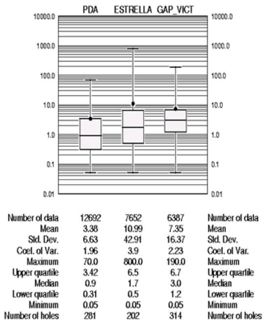
Figure 14-49 PDA Project - Boxplots of Silver Grade Composites – Capped – Within Mineralized Zones
