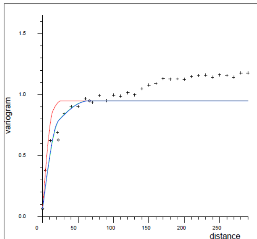
Figure A-11. Copper Variograms – Oxide – La Yaqui Grande
