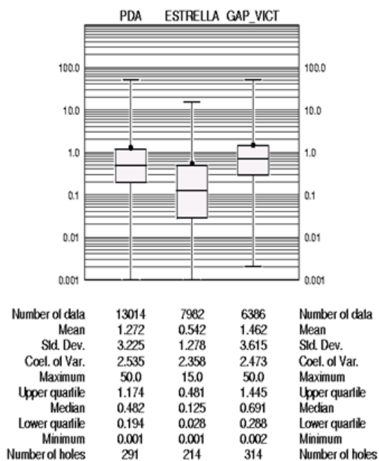
Figure 14-48 PDA Project - Boxplots of Gold Grade Composites – Capped – Within Mineralized Zones
