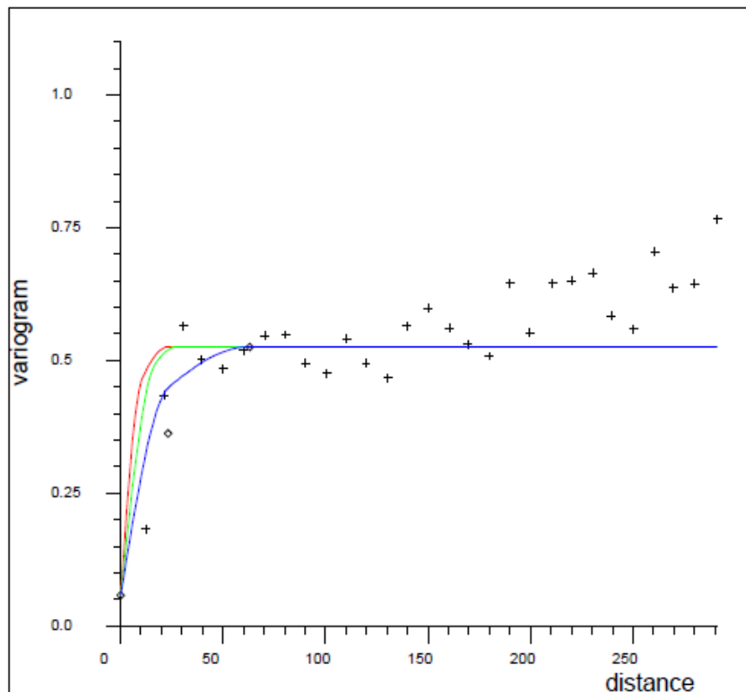
Figure A-7. Silver Variograms – Higher-Grade Silver Zone 3 – La Yaqui Grande
