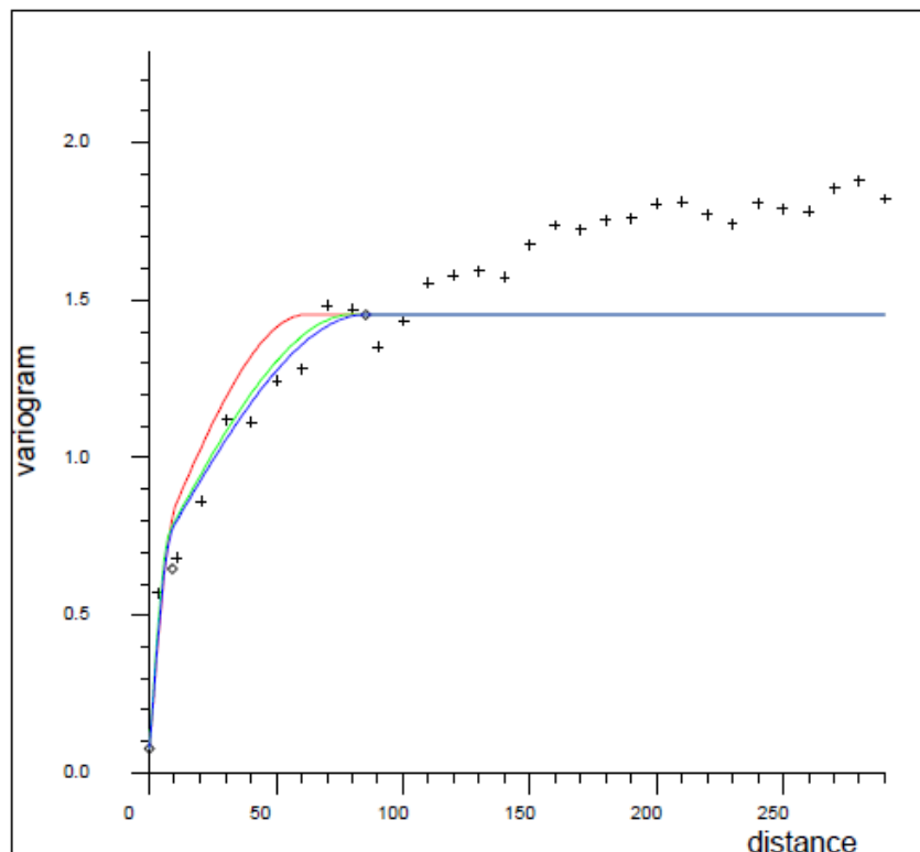
Figure A-8. Silver Variograms – Outside Higher-Grade Silver Zones 1+2+3 – La Yaqui Grande
