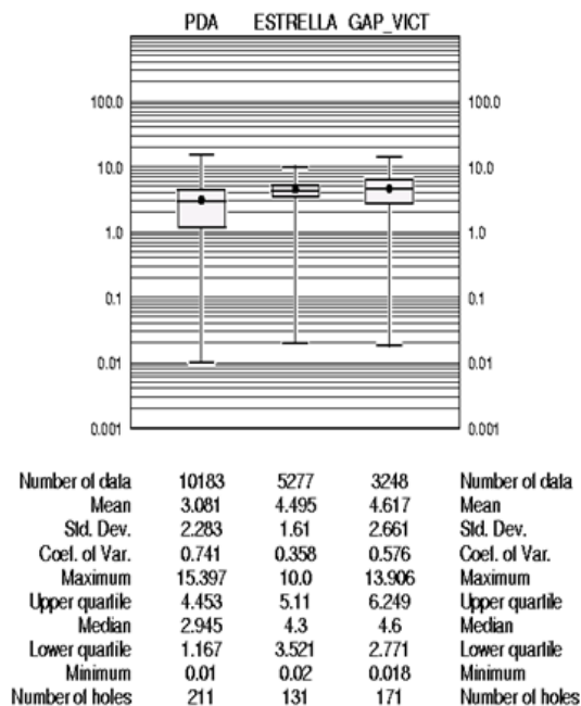
Figure 14-47 PDA Project - Boxplots of Total Sulphur Grade Composites – Un-Capped – Within Mineralized Zones
