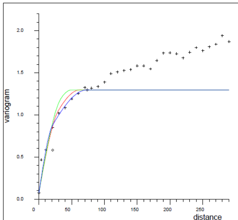
Figure A-4. Gold Variograms – Outside Higher-Grade Gold Zones 1+2+3 – La Yaqui Grande
