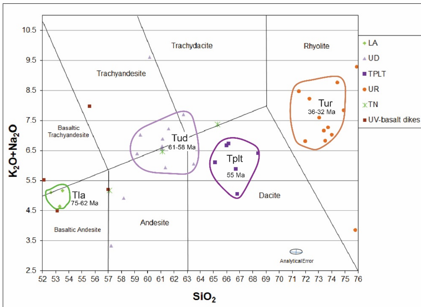
Figure 7-2 Total Alkali Silica (TAS) Diagram Showing the Compositional Variation through Time for the Mulatos Rocks.
