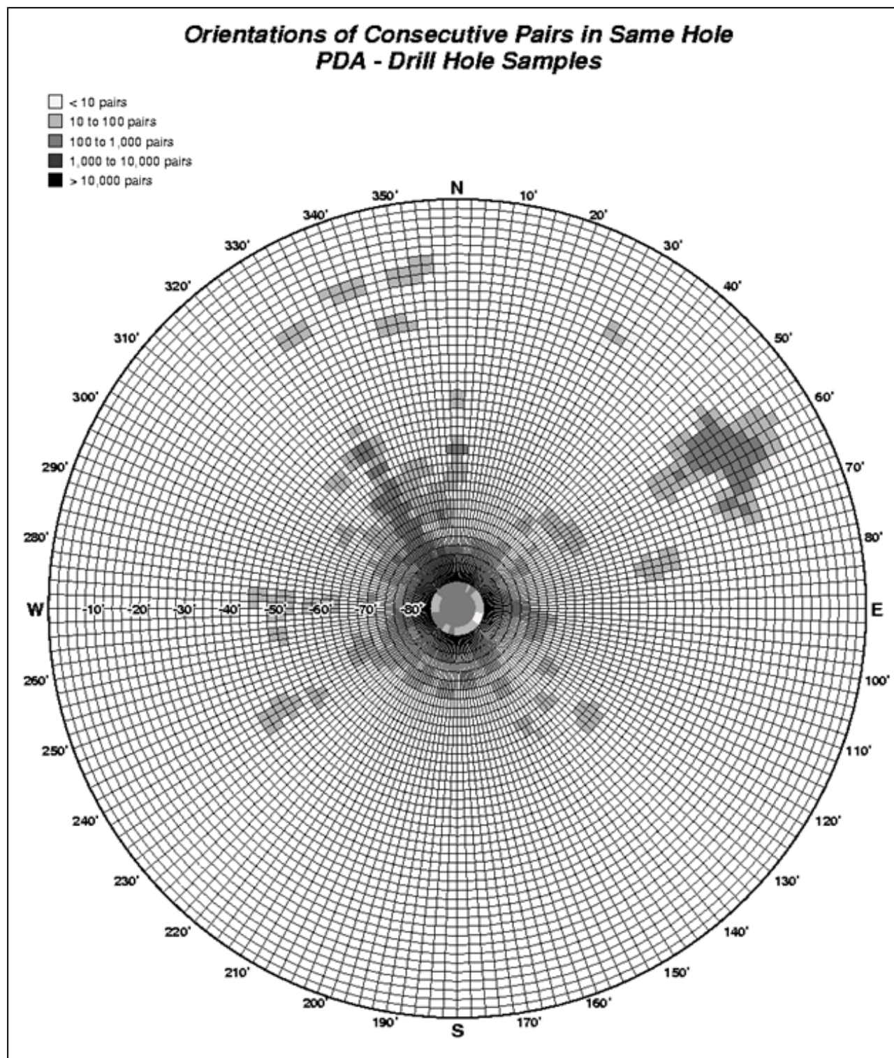
Figure 14-35 PDA - Drill Hole Orientation – Stereonet
