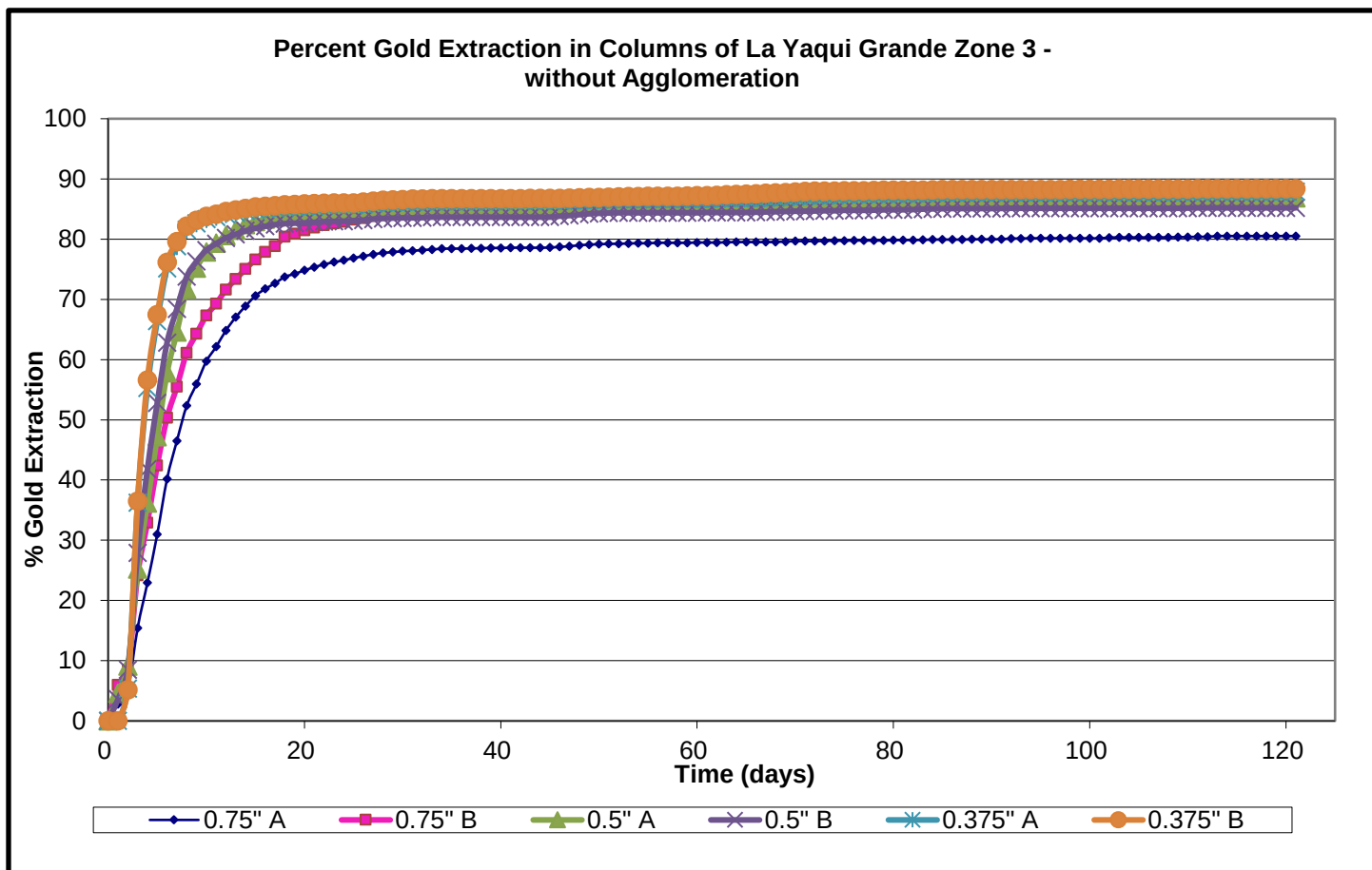
Figure 13-8 La Yaqui Grande Zone3 Columns without Agglomeration
