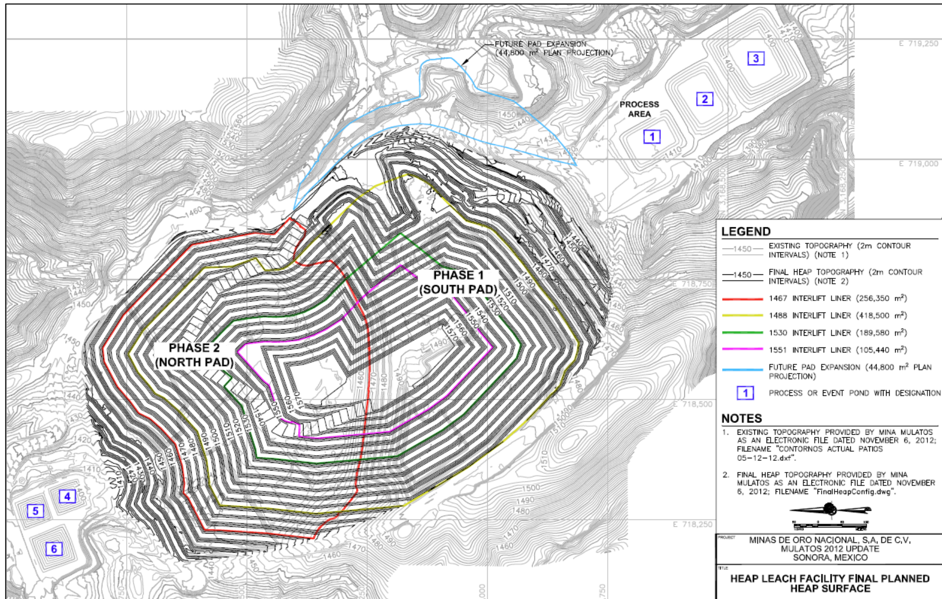
Figure 17-2 Mulatos Phase 1 and 2 Heap Leach Final Design
