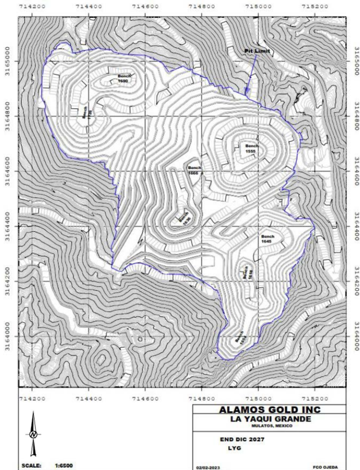
Figure 16-10 La Yaqui Grande Pit Plan, End of 2027
