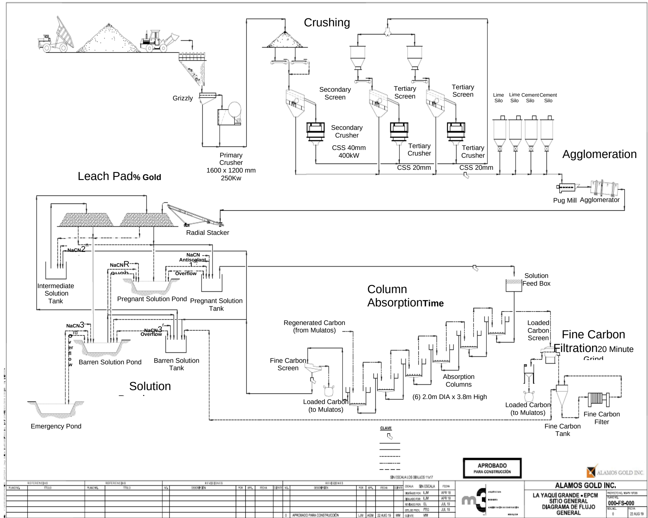
Figure 17-4 Yaqui Grande Heap Leach Overall Flowsheet
