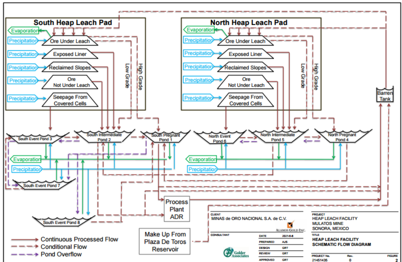
Figure 20-2 Mulatos Flow Diagram of Heap Leach Facility
