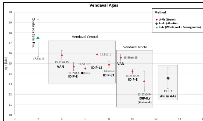
Figure 4 - Geochronology ages at Vendaval.
