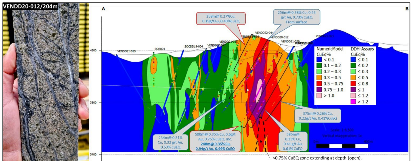
Figure 4 - Long Section view to NW of Vendoval Central with CuEq grades after phase IV, Lefthand image shows typical 'EMP' core.
