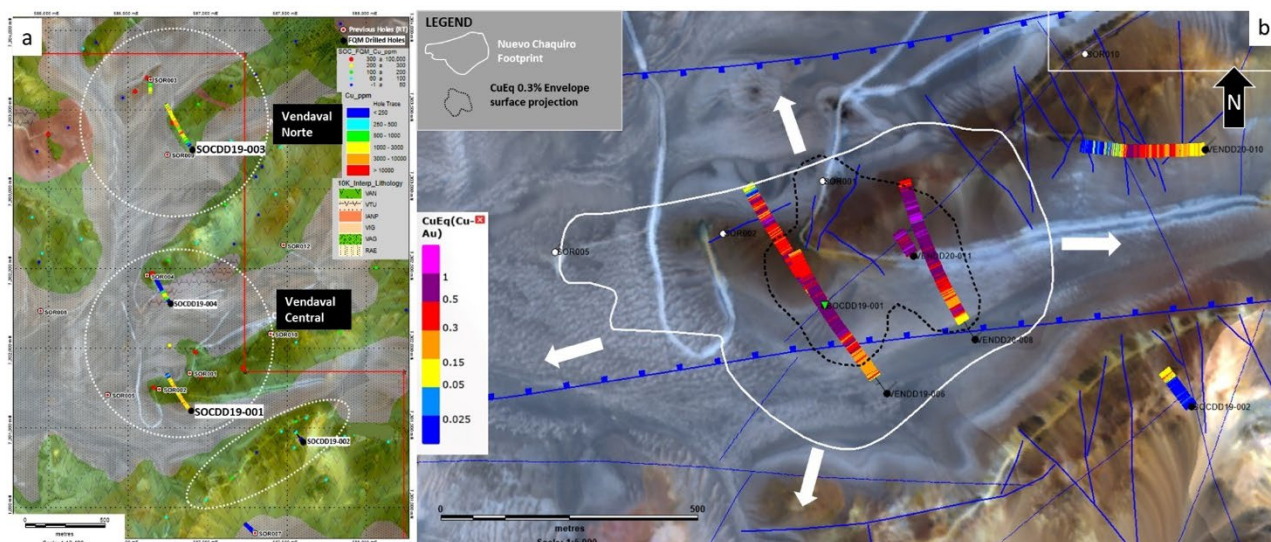
Figure 3 - (a) results after Phase I showing the main two porphyritic centres identify on Vendaval; (b) Vendaval Central in comparison with other porphyries copper-gold (Nuevo Chaquiro, Colombia), showing the potential open areas, after drilling Phase II.
