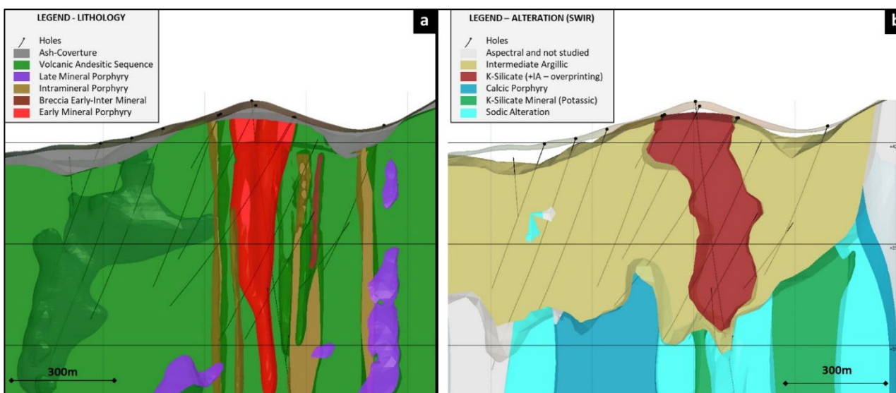
Figure 7 - Long section along Vendraal Central deposit (a) 3D lithological model showing the different pulses intruding the volcanic andesitic hosting sequence. (b) 3D Model Alteration - SWIR, modelled from the integration of geochemistry + SWIR data from TerraSpec to define the alteration domains (Cernuschi, 2023).
