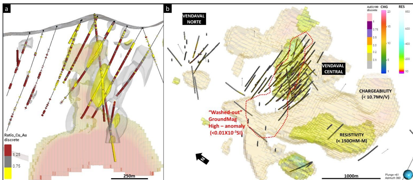
Figure 10- Section on the core of Vendaval Central view to the E, with 3D Magnetic (constrain – Susmag) model and Ratio Cu/Au values (filtered with values > 0.15% Cu content), on grey ratio ~1 and on yellow ratio ~ 0.75 (higher gold rather than copper), is evident the continuity in depth. (b) – Oblique view of Vendaval (including Norte & Central), with geophysical response on Central body (mid-high magnetic with voiding zone of chargeability (mid-low values) and High resistivity related to sheeted quartz veining density >5 vein/m related to main ore Phase.
