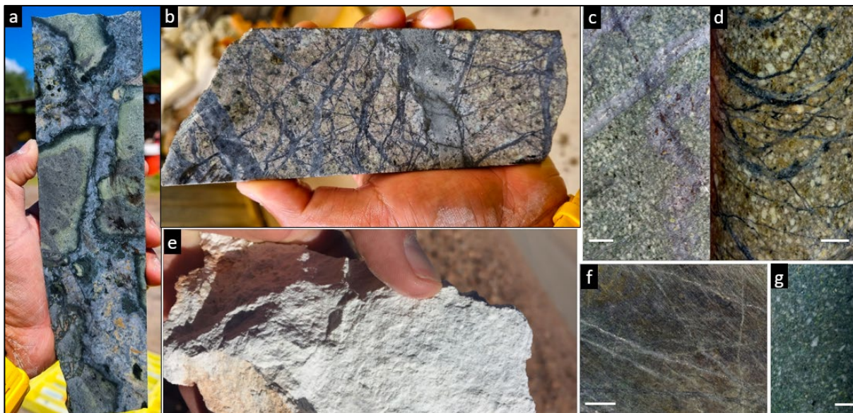
Figure 6 - Mosaic from core with relevant alteration types (a) Garnet-pyroxene-chlorite alteration (calcic assemblage). (b) Diorite porphyry (EMP) with strong potassic feldspar - biotite (potassic-silicate alteration). (c,d) Smectite - chlorite - illite alteration (Intermediate argillic assemblage with variations). (e) Pervasive strong steam heated silica - kaolinite alteration with relicts pyrophyllite - dickite. (f) Hornfelsized volcanics (silica-magnetite - biotite - chlorite). (g) Propylitic alteration (chlorite - epidote - calcite).
