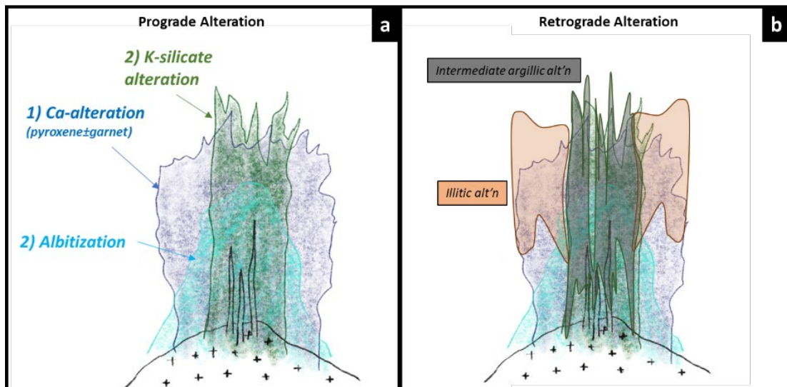
Figure 5 - Alteration Model – evolution of Vendaal deposit (a) Prograde alteration and (b) retrograde alteration from Cernuschi et al., 2023a
